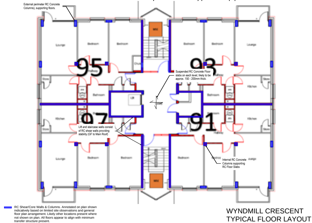
Figure 6: Diagram of typical floor plan
