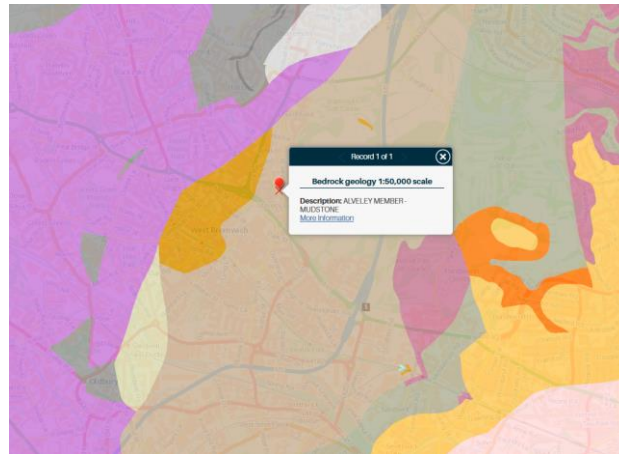
Figure 2. Bedrock Geology
