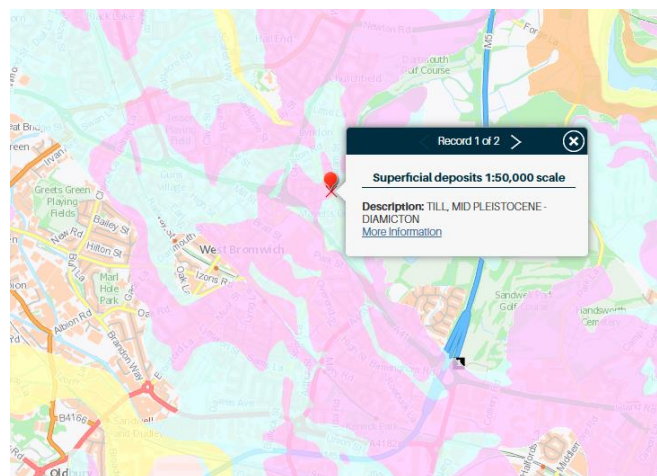
Figure 3. Superficial Geology
