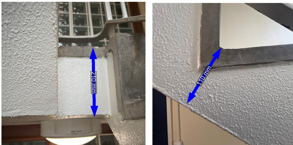
Figure 15 and 16: Stair stringer and RC slab
