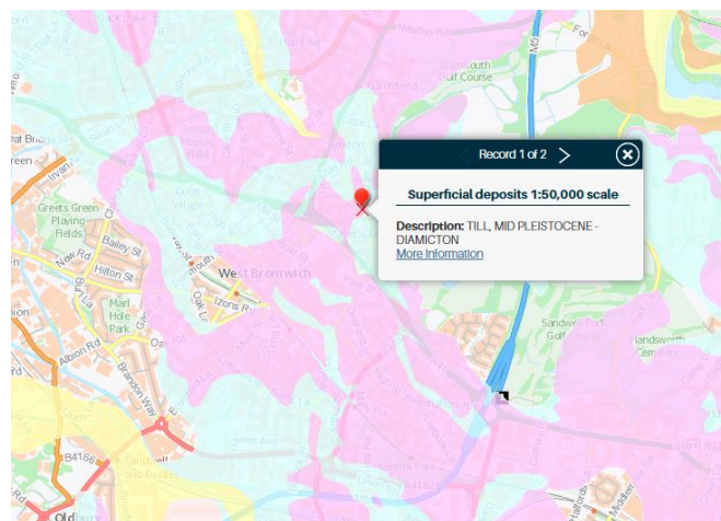
Figure 3. Superficial Geology
