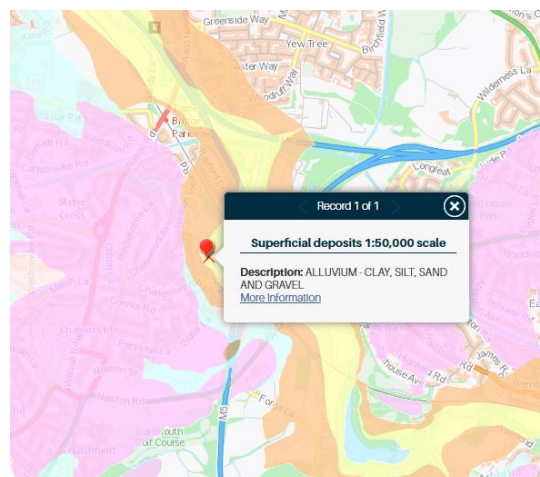
Figure 3. Superficial Geology
