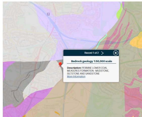
Figure 2. Bedrock Geology
