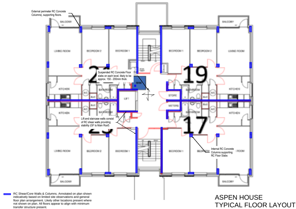
Figure 6: Diagram of typical floor plan
