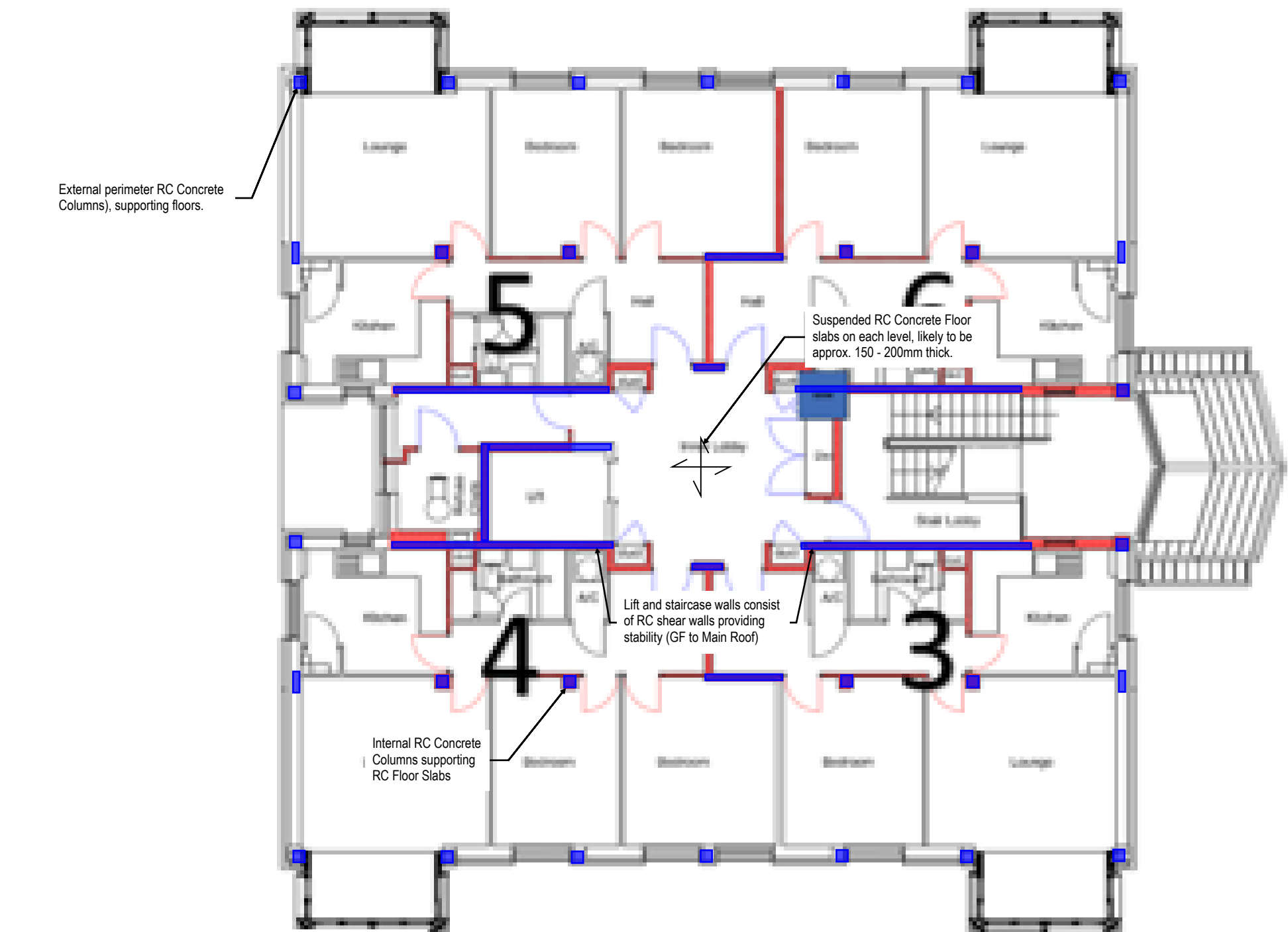
MACAULEY HOUSE TYPICAL FLOOR LAYOUT
