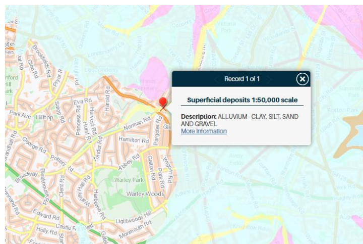
Figure 3. Superficial Geology
