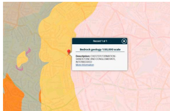
Figure 2. Bedrock Geology
