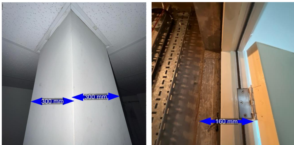
Figure 15 and 16: RC Column and Wall Size
