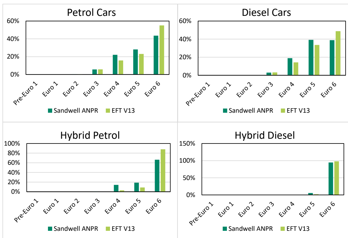
Figure 3-6 – Car Euro Classification, ANPR and EFTv13, 2022
