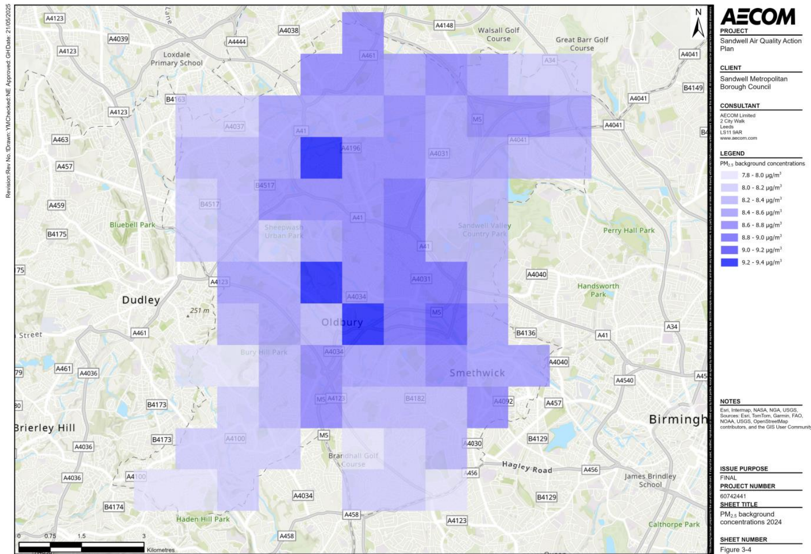
Figure 3-4 – Background PM 2.5 Concentrations in Sandwell
